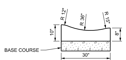
CURB AND GUTTER, TYPE G, MODIFIED N.T.S.
