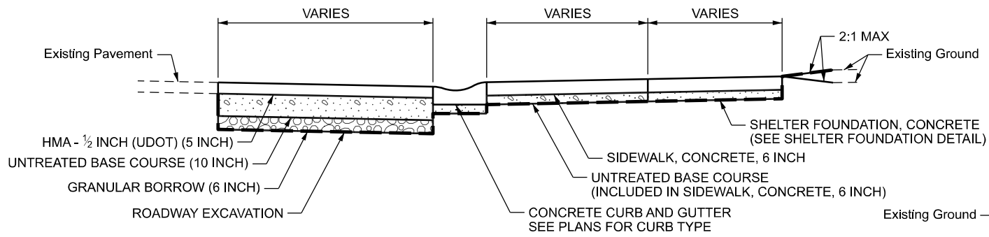
PARK CITY COMMERCIAL COLLECTOR PAVEMENT SECTION N.T.S.
