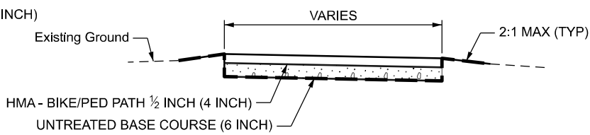
ASPHALT PATHWAY PAVEMENT SECTION N.T.S.
