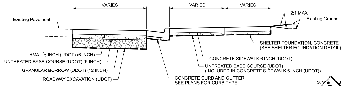
UDOT STATE ROUTE PAVEMENT SECTION N.T.S.
