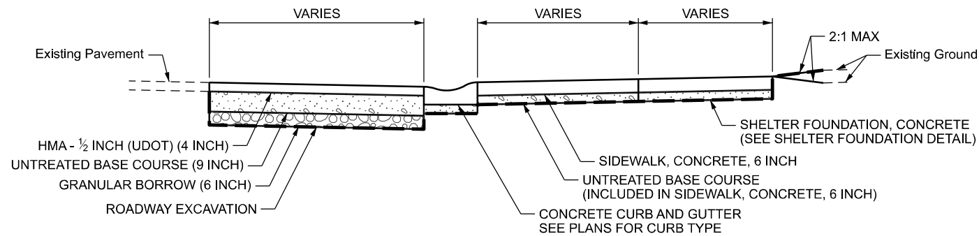
PARK CITY RESIDENTIAL COLLECTOR PAVEMENT SECTION N.T.S.
