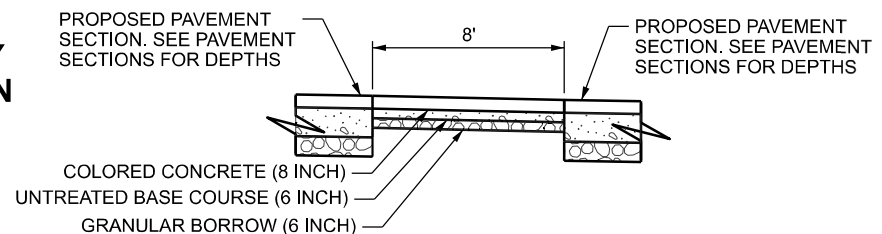
COLORED CONCRETE CROSSWALK SECTION N.T.S.
