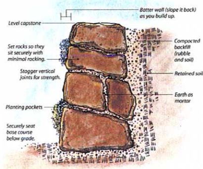
Maximum 6' stacked rock wall
