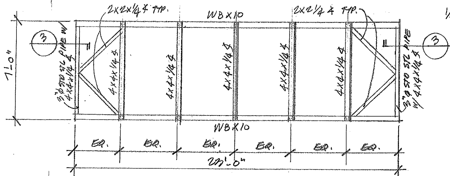
2 DETAIL 1" = 1/20"
