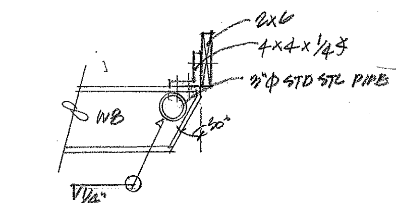
3 DETAIL 1" = 1/20"
