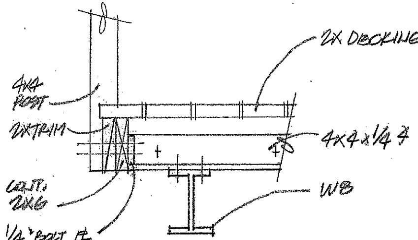
2 DETAIL 1" = 1/20"
