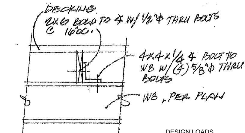
1 DETAIL 1" = 1/20"
