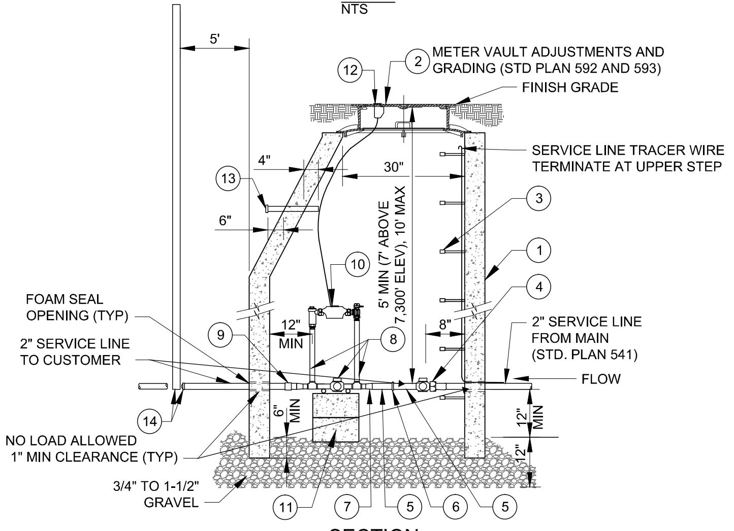
SECTION NTS
