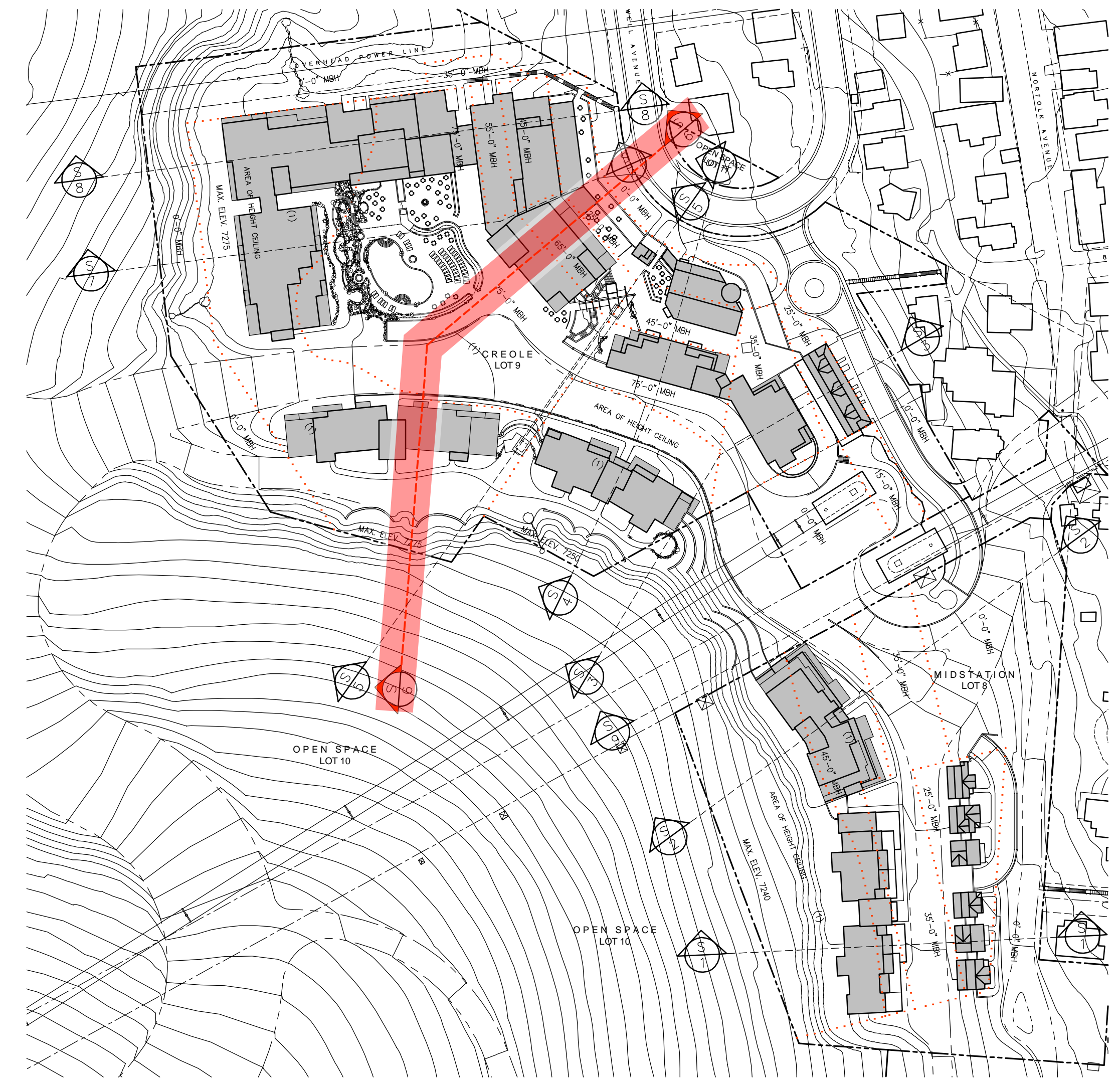
KEY PLAN
