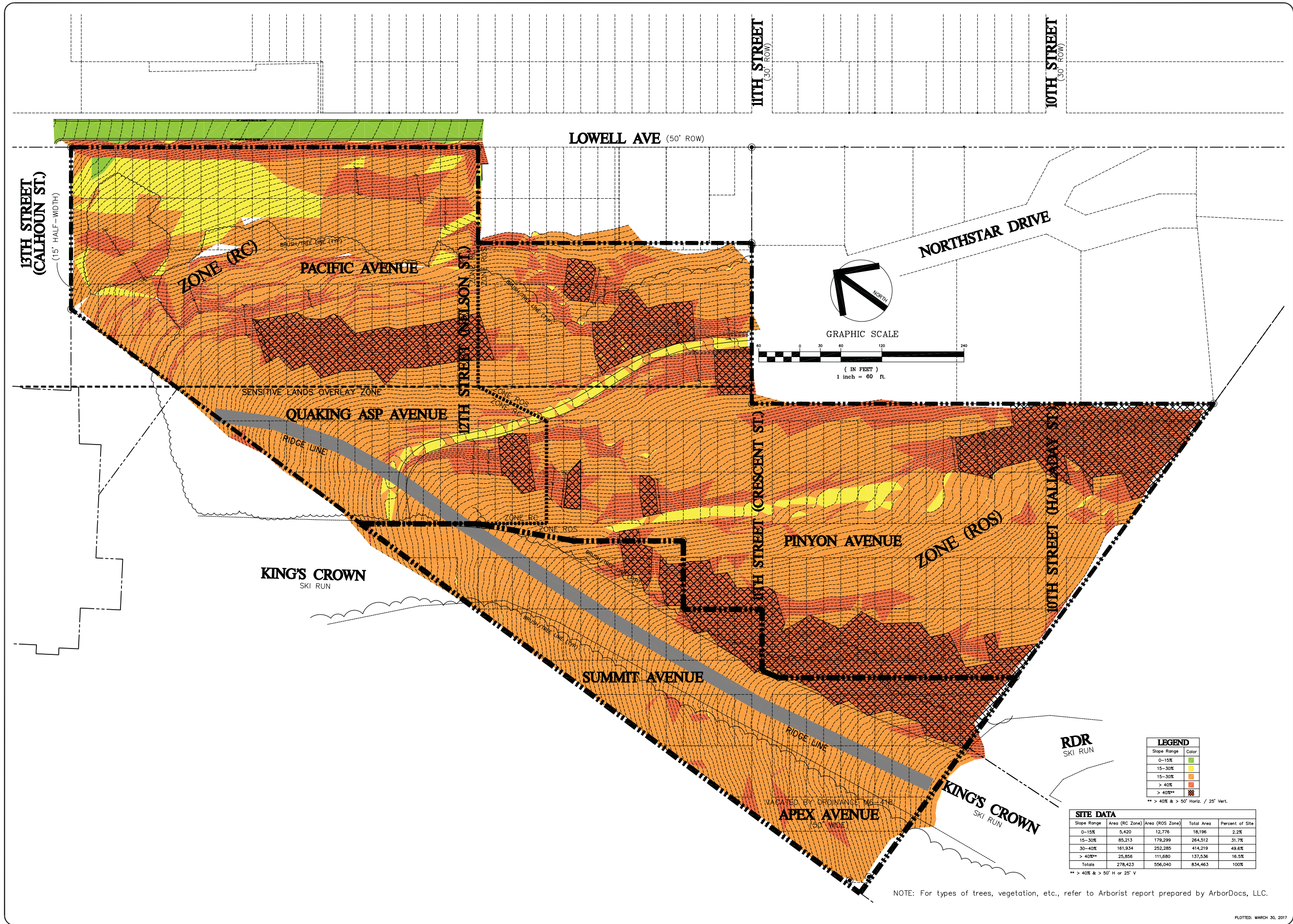
Appendix K {Existing Slope Map}
