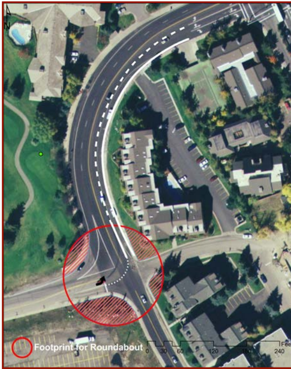
Figure 5-3: Intersection Improvement, Silver King Drive and Empire Avenue
